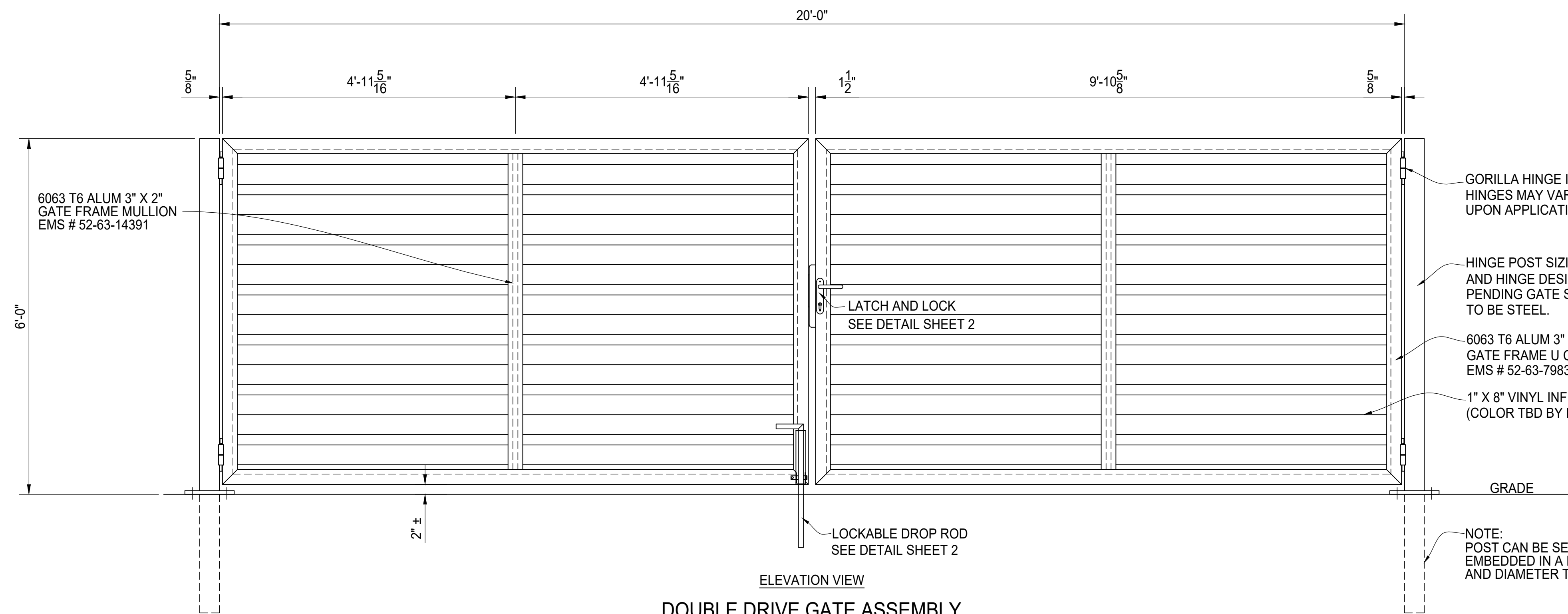
DOUBLE DRIVE GATE ASSEMBLY SEE DETAIL SHEET 2 FOR HINGE, LATCH AND DROP ROD
