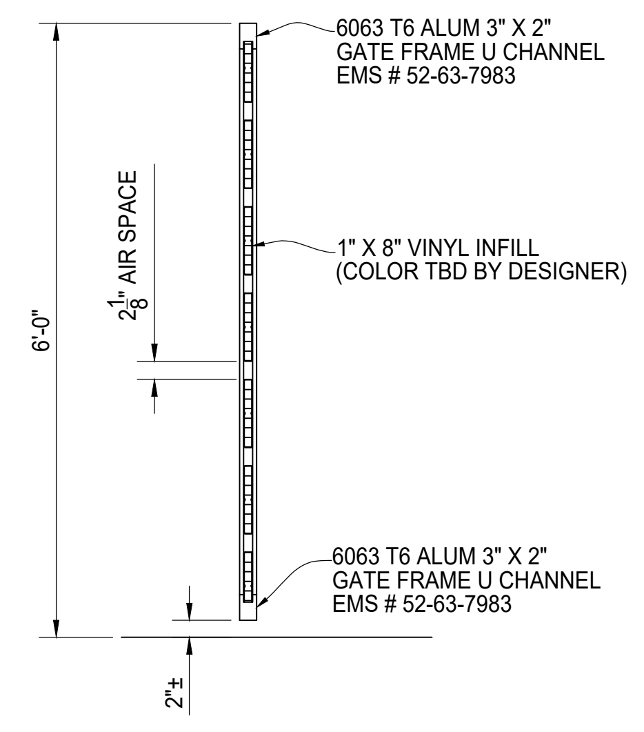
SIDE VIEW
