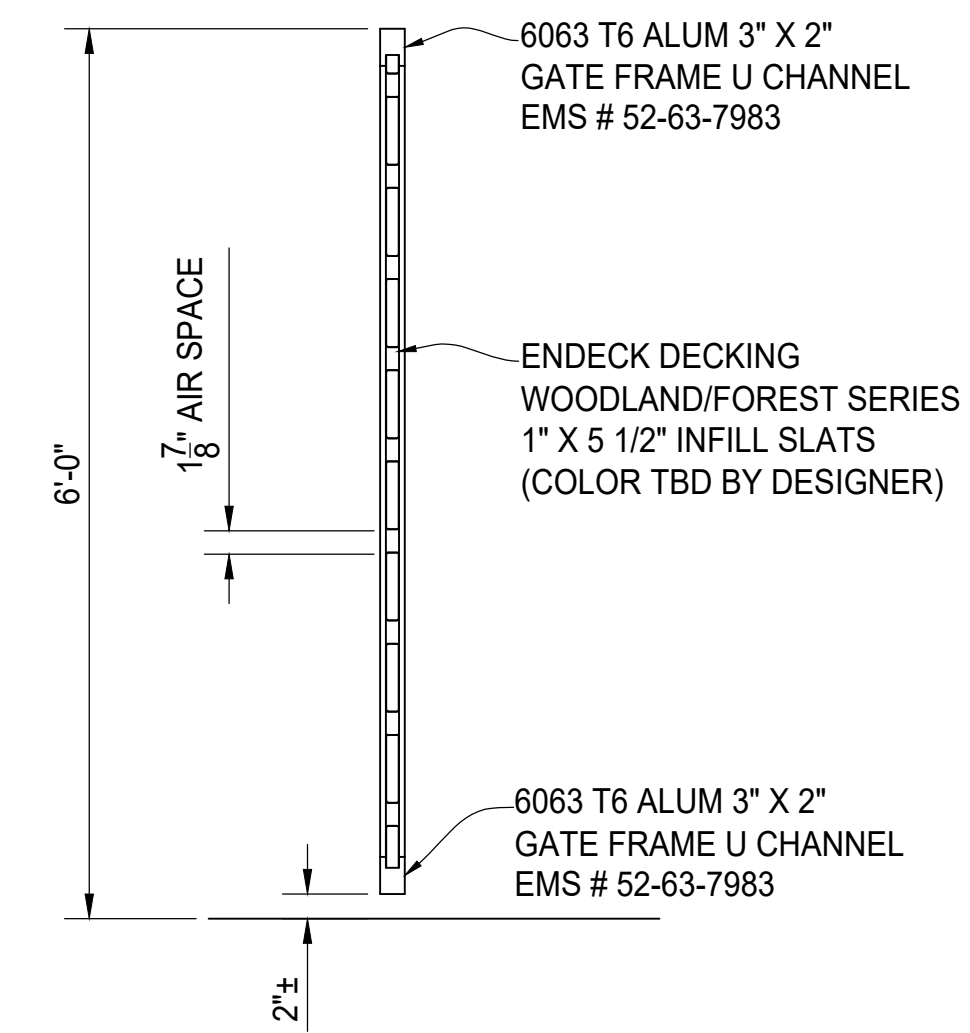
SIDE VIEW
