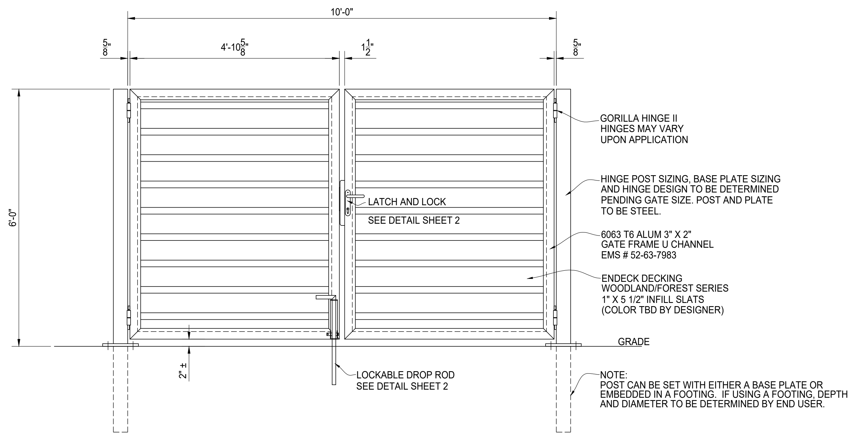
ELEVATION VIEW
