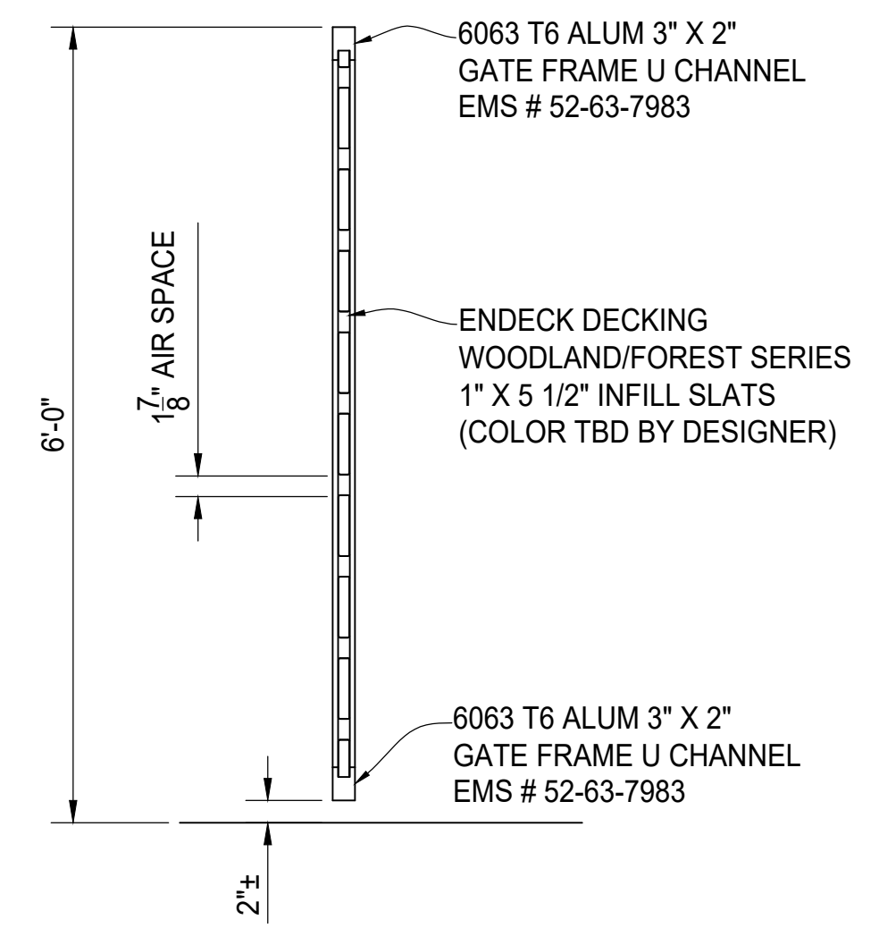
SIDE VIEW
