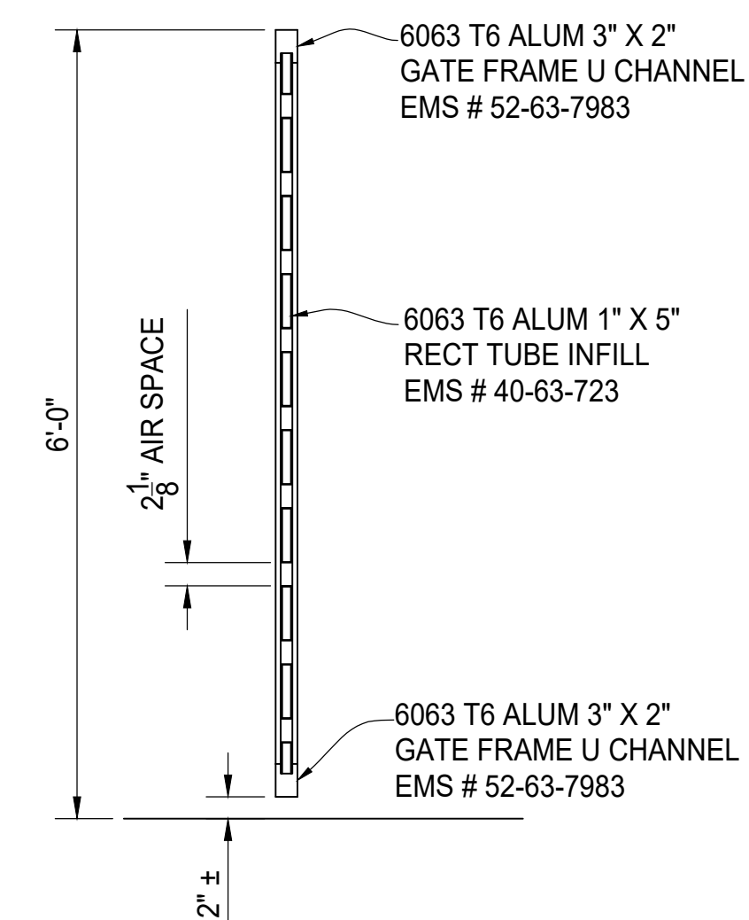
SIDE VIEW GATE SECTION
