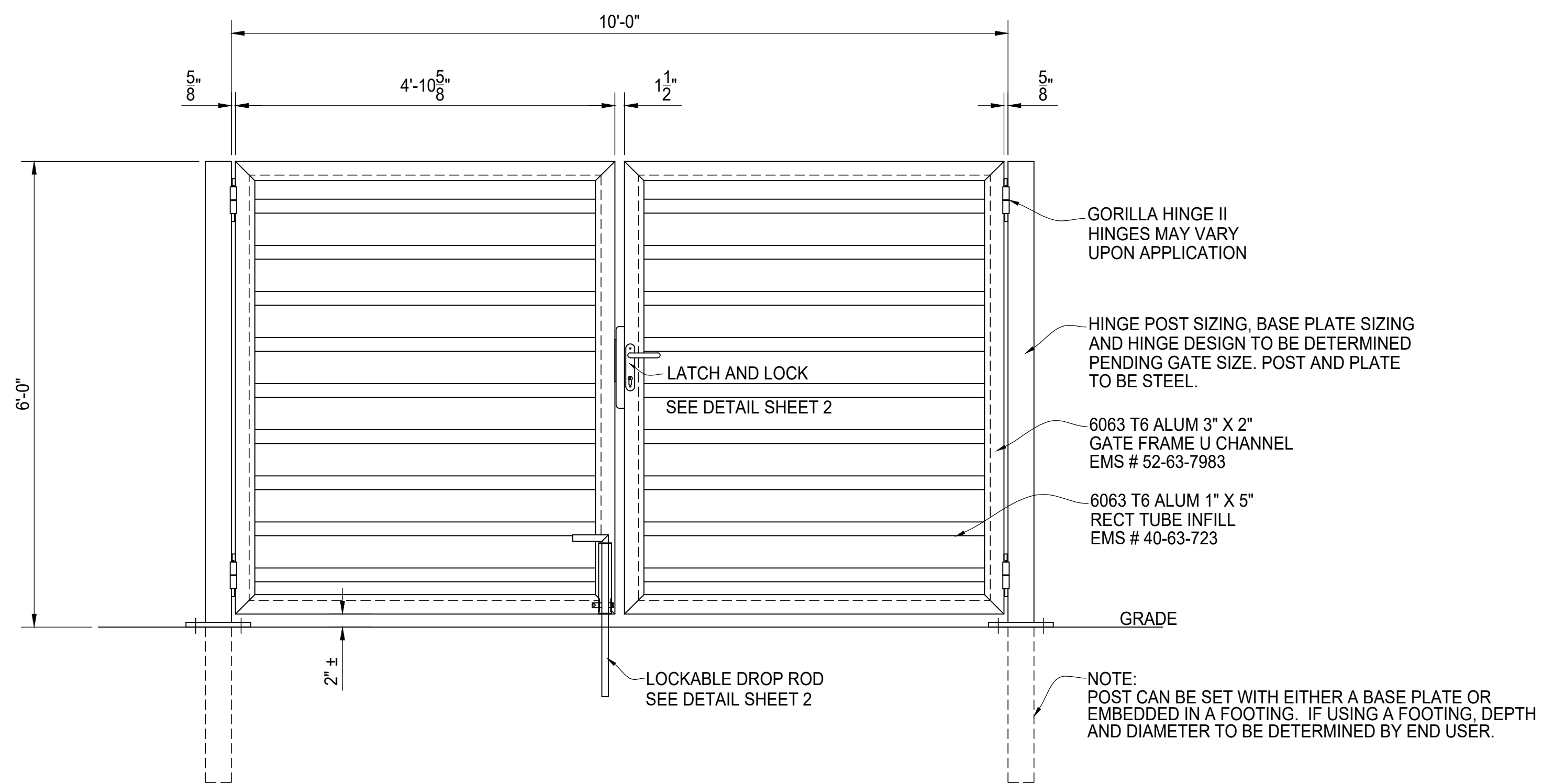
ELEVATION VIEW
