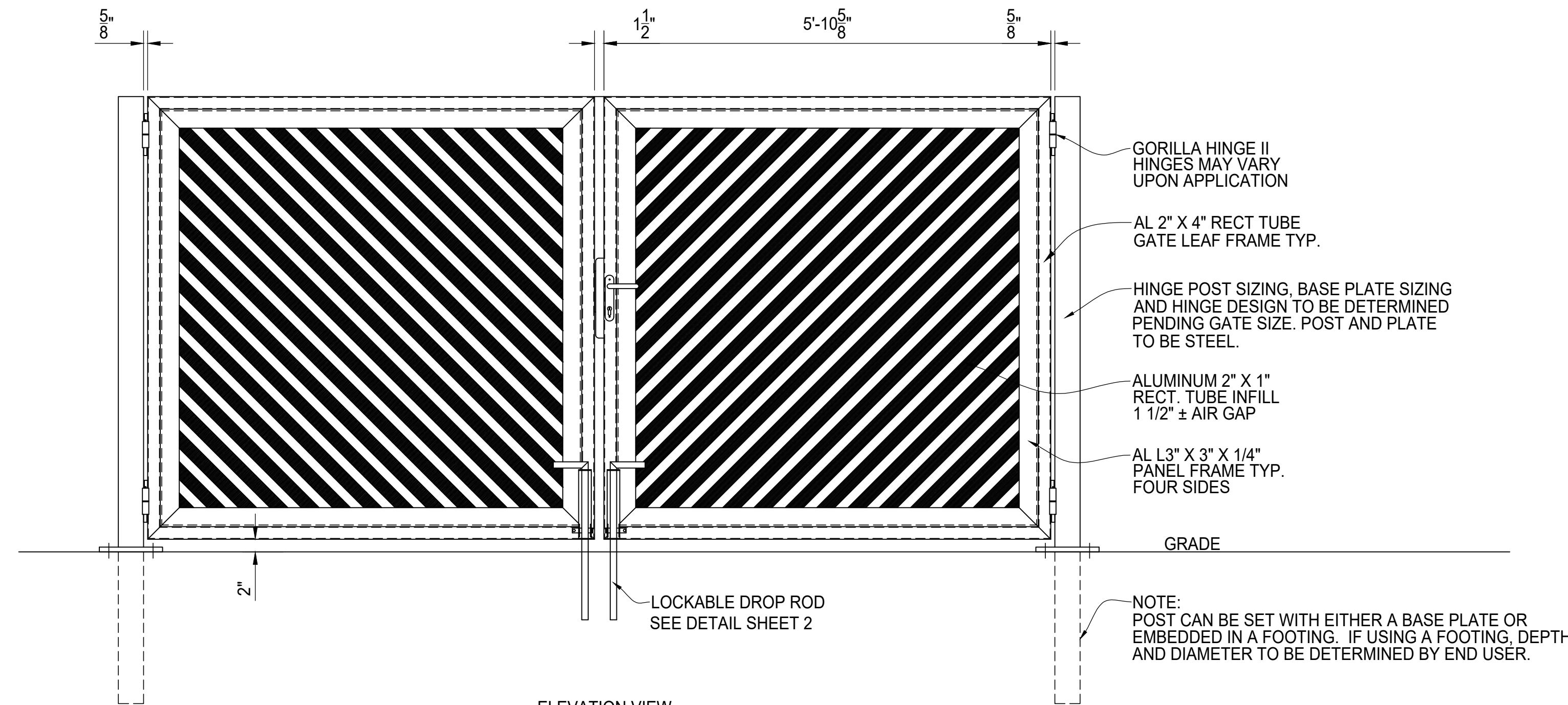
ELEVATION VIEW
