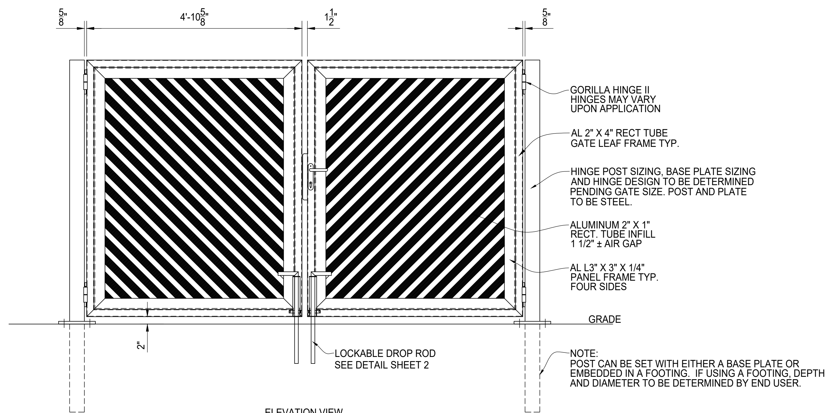
ELEVATION VIEW
