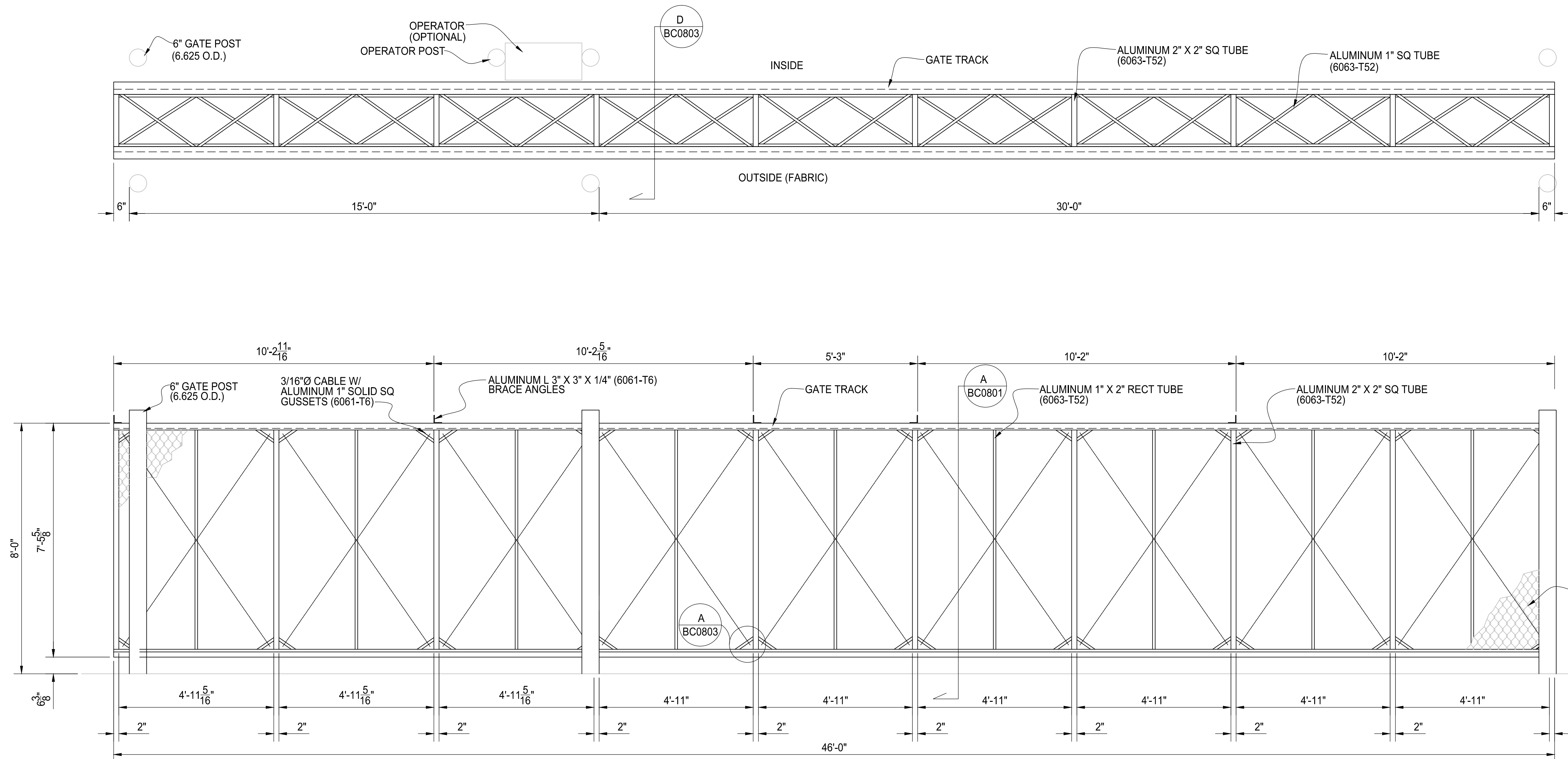
ELEVATION VIEW OF ALUMINUM BOX FRAME CANTILEVER OUTSIDE LOOKING IN, OPERATOR NOT SHOWN THIS VIEW
