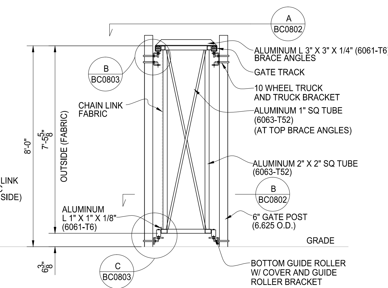
SECTION VIEW OPERATOR NOT SHOWN THIS VIEW
