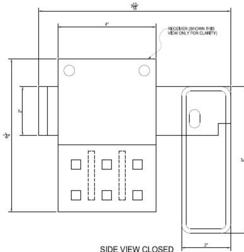
SIDE VIEW CLOSED
