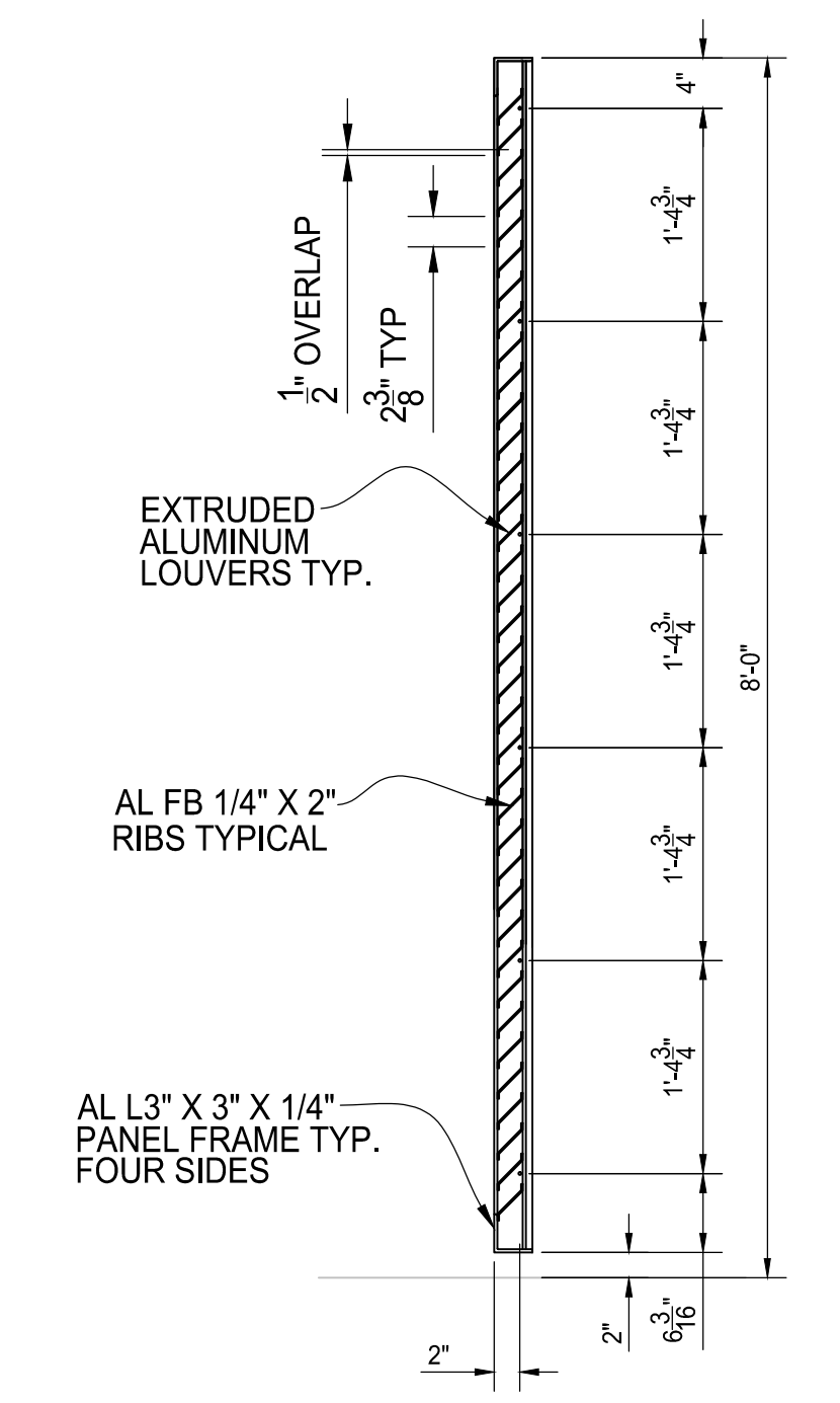
B TYPICAL PANEL SECTION
