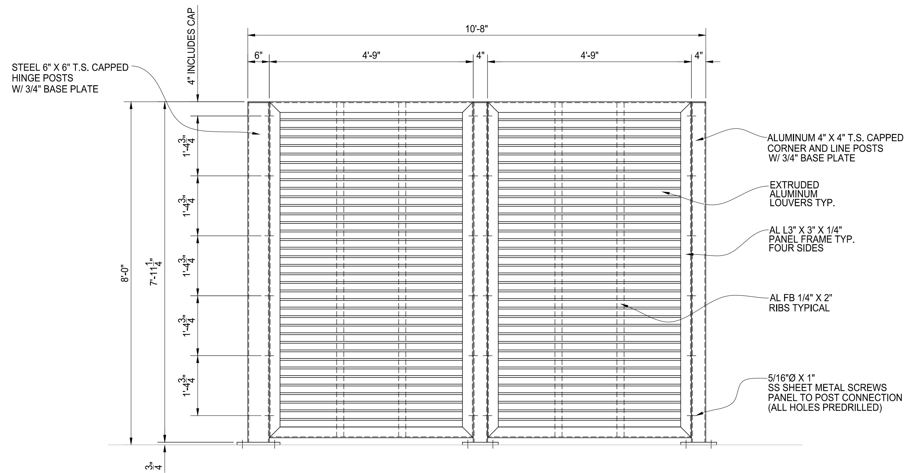
A ELEVATION VIEW
