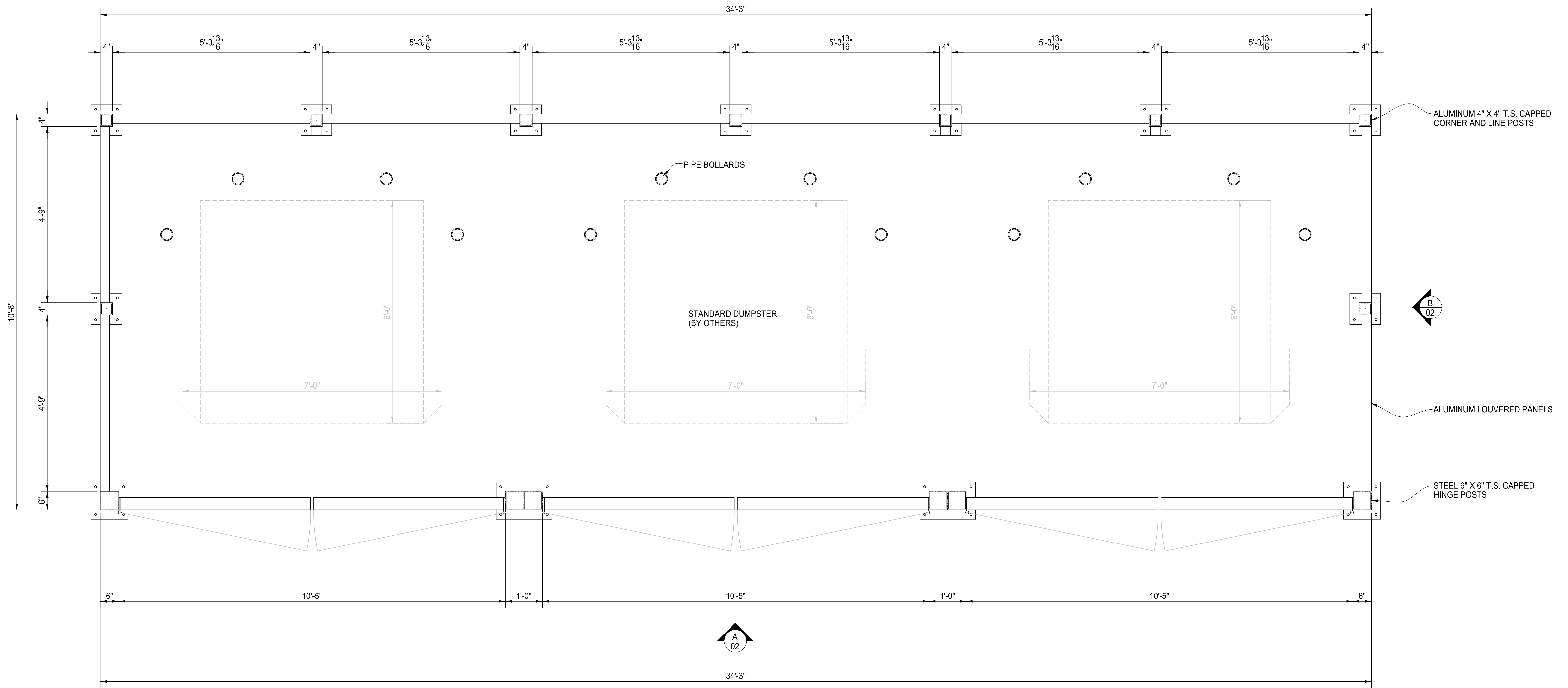
PLAN VIEW @ DUMPSTER ENCLOSURE
